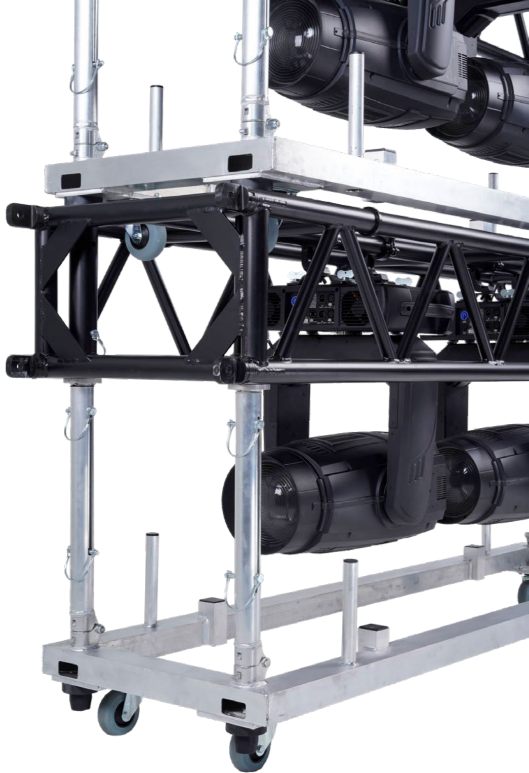
Rotatable forks for curving.
