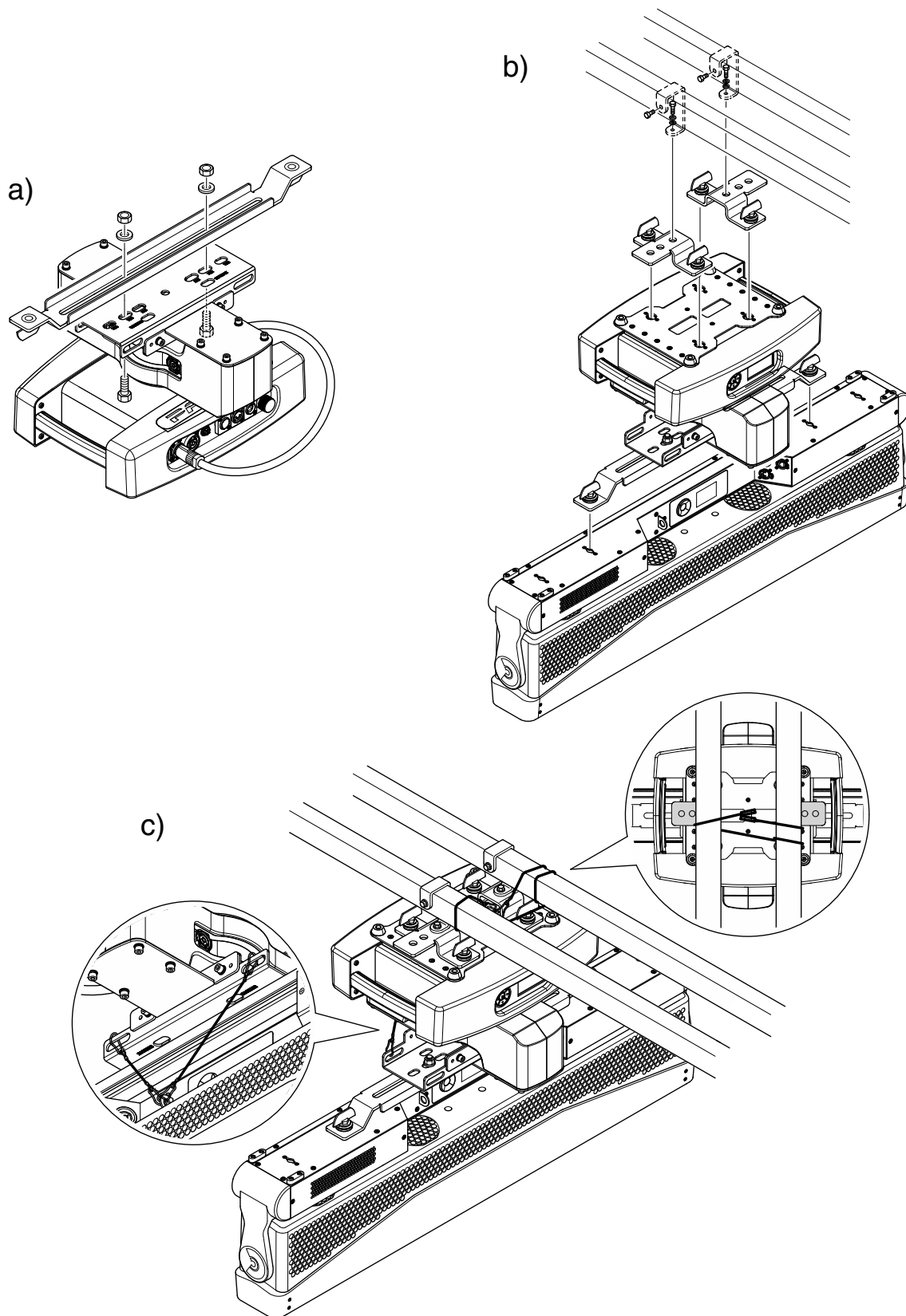
Installing the fixture - Fig. 2
