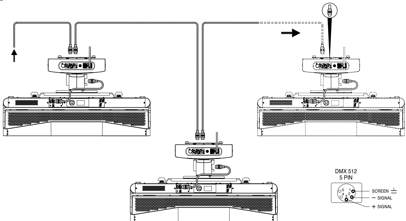
Connecting to the control signal line (DMX) - Fig. 6
